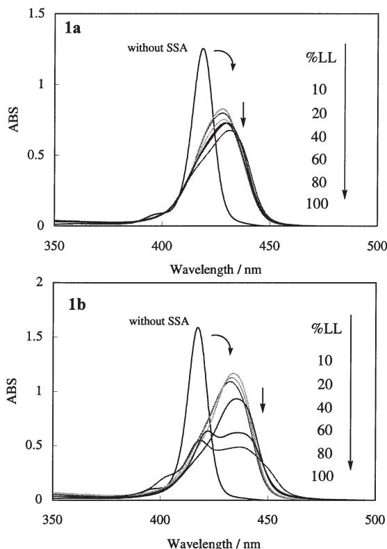
Figure 2. Absorption spectra of 1a and 1b at various %LL for aqueous SSA solution.
