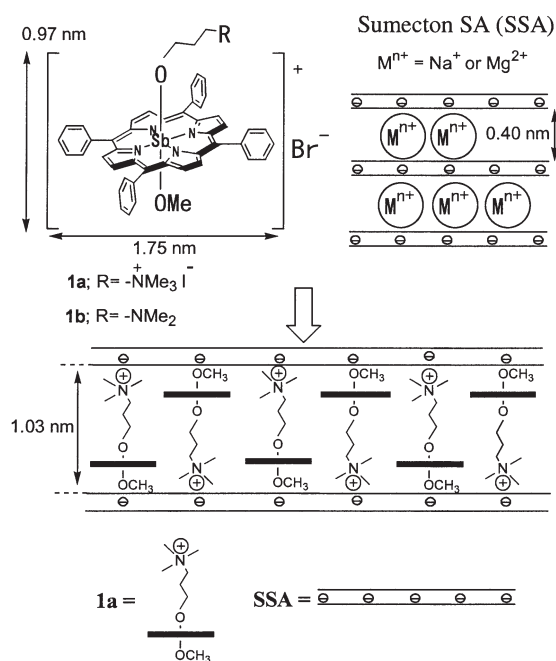
Figure 1. Schematic diagram of possible layered structure.
